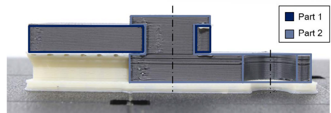
Fig. 1. Additively manufactured joint with soluble support
