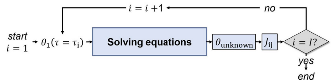
Fig. 4. Procedure for determining the unknown angles of the joints through solving the vector loop equations
