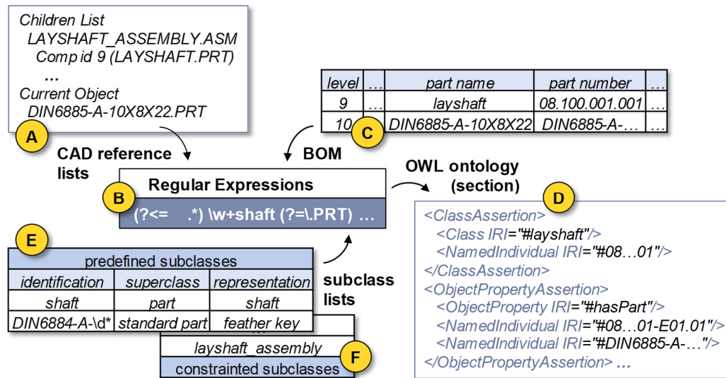
Figure 3. Automated generation of ontologies
