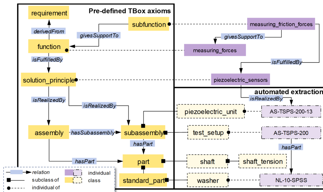
Figure 5. Example ontology with automated-extracted elements of the test-rig
