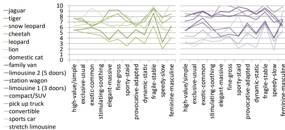
Fig. 4. Selected impressions profiles of cats' (left) and cars' variations (right) conducted with ACADE [14]
