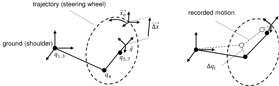
Figure 5 Kinematical dummy of the demonstrator
