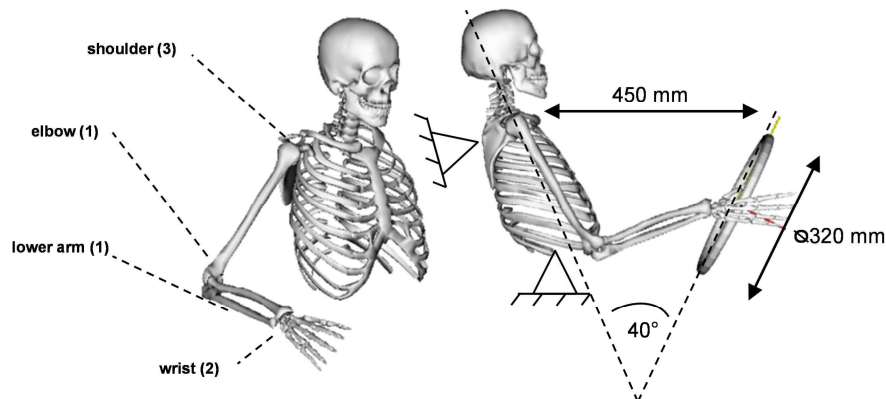
Figure 1 Demonstrator (left: degrees of freedom, right: dimensions)
