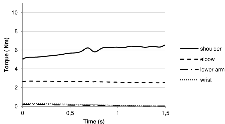
Figure 7 Joint torques (determined using inverse dynamics)
